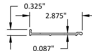
16 SILL TRIM BASE 6063-T5
