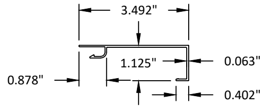
71 1 1/8" X 3 1/2" COVER 6063-T5
