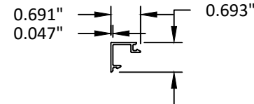
14 VENT SNAP COVER 6063-T5
