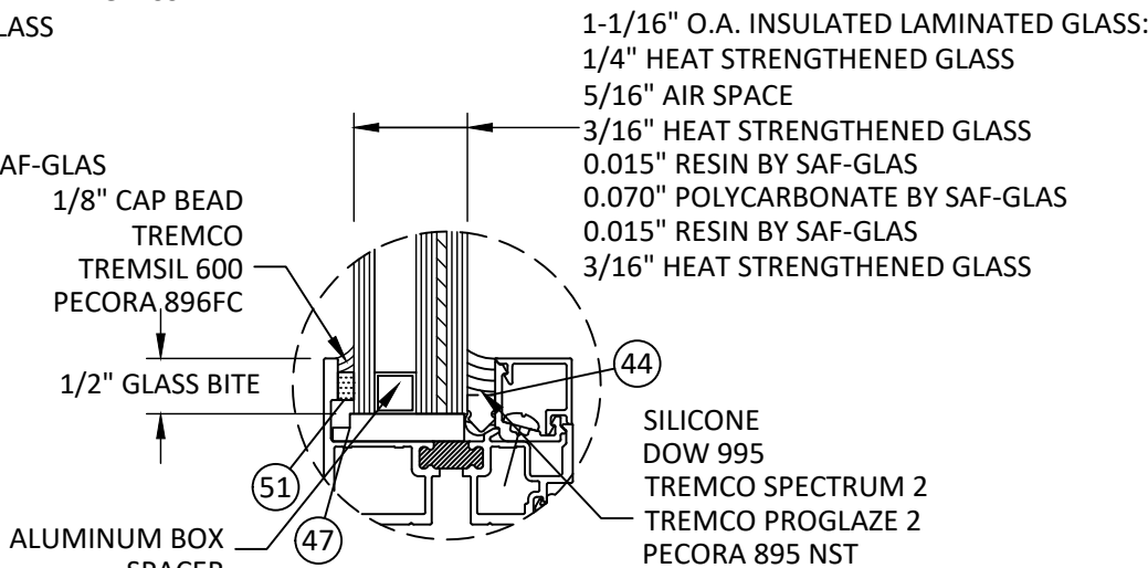
GLAZING DETAIL B1
