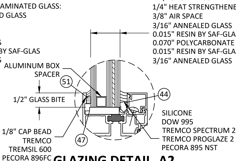
GLAZING DETAIL A2
