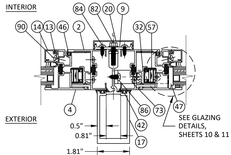
Y9 HORIZONTAL SECTION STACK MULLION - TYP. PROJECT OUT TO PROJECT OUT
