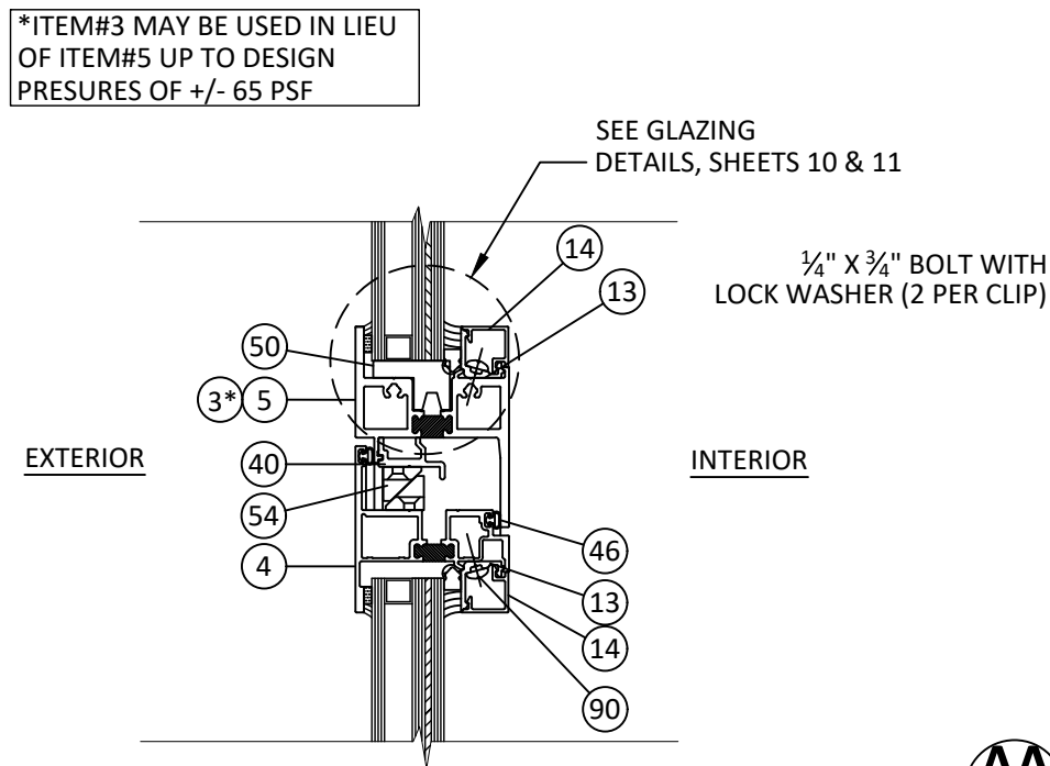
V9 VERTICAL SECTION INTEGRAL MULLION-TYP. FIXED OVER PROJECT OUT
