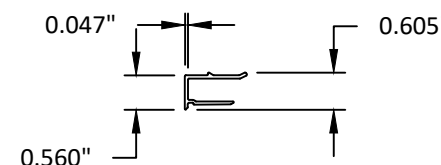
22 FIXED GLASS STOP COVER 6063-T5
