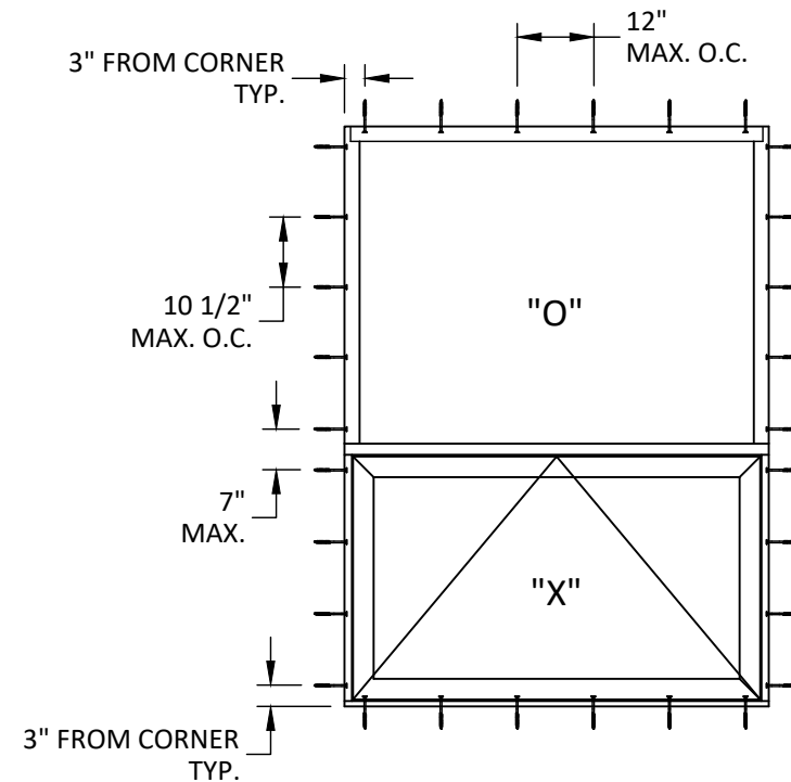
ANCHOR LAYOUT ALL INSTALLATIONS
