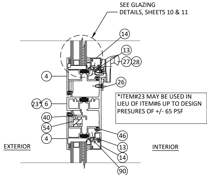
W9 HORIZONTAL SECTION PROJECT OUT - PROJECT OUT
