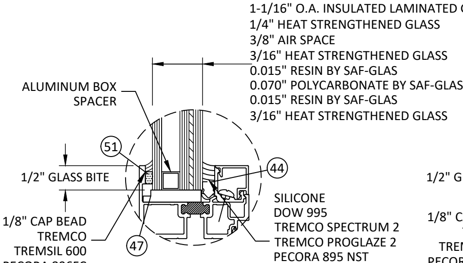
GLAZING DETAIL B2
