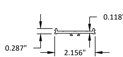
9 PRESSURE BAR 6063-T5
