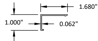
69 1" X 1 11/16" COVER 6063-T5
